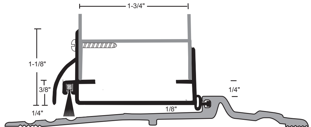
Designed for use on standard 3/4" undercut door used with NGP 896 V, N, or S ADA compliant threshold as shown
