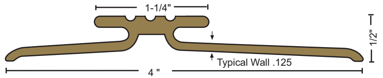
442BR 2.01 lbs./ft.
