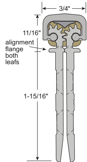
Frame leaf covers butt hinge preps
