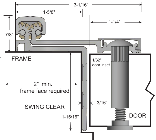
Frame leaf covers butt hinge preps Concealed fastener cover on door leaf
