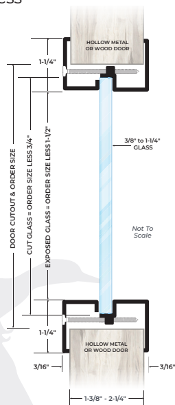
Designed for Use on 1 3/4" Thick Doors Manufactured Within Door Industry Tolerance of +/- 1/16".
