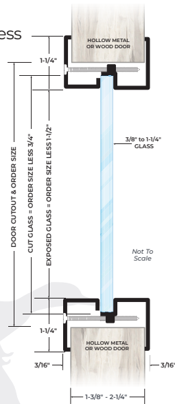
Designed for Use on 1 3/4" Thick Doors Manufactured Within Door Industry Tolerances of +/- 1/16".
